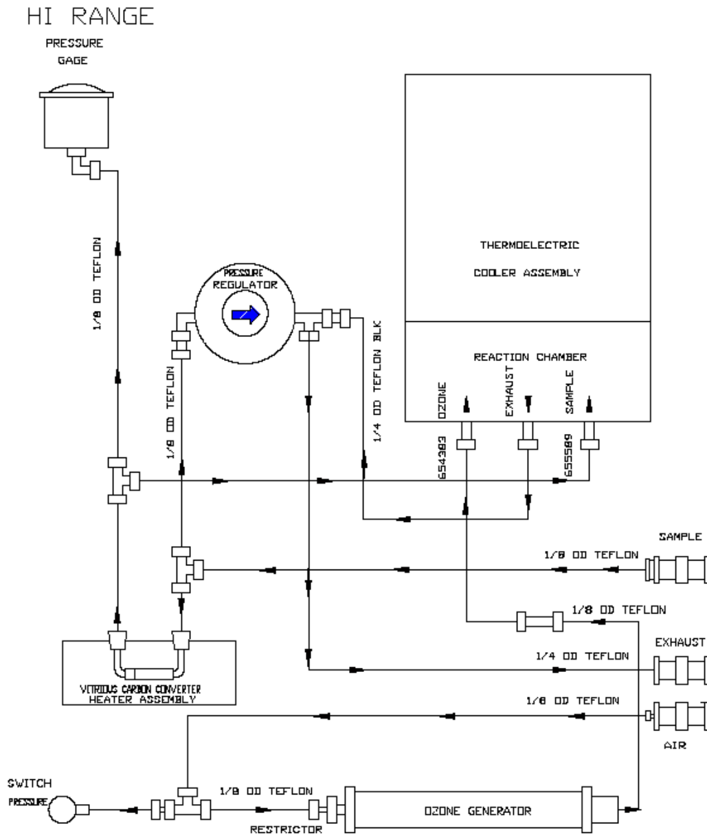
Drawing 1-3 Flow Diagram, Hi Range
